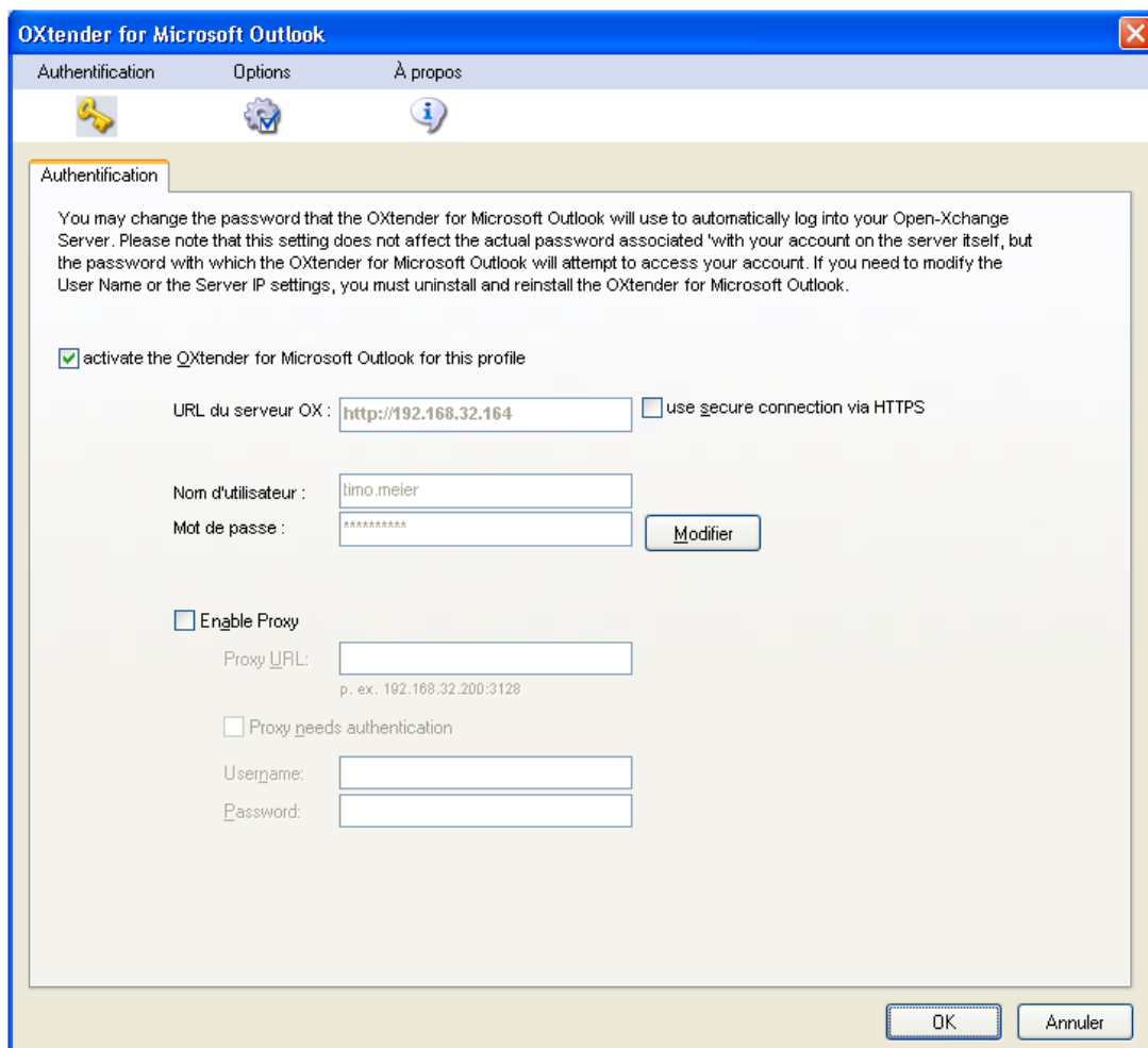
Figure 4.2. Onglet Authentification
