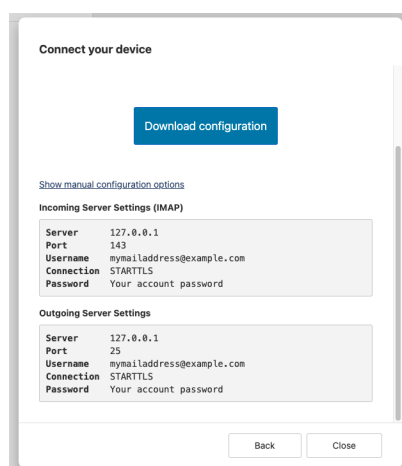
Figure 2: example wizard
