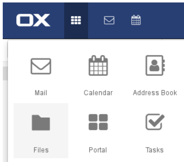
Figure 2: Files App
