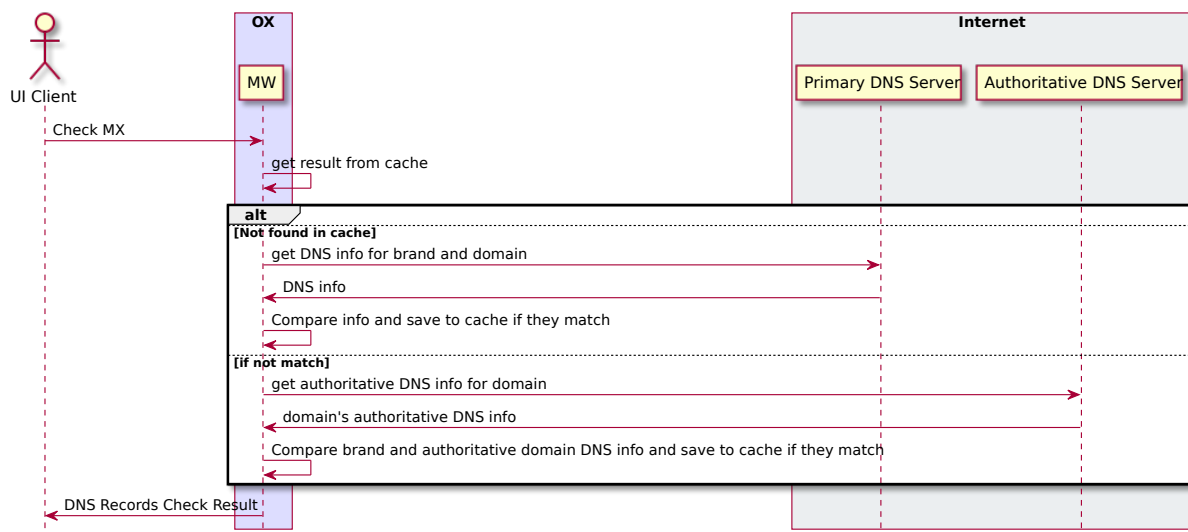
Figure 1: PlantUML 1
