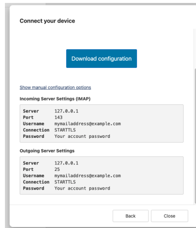
Figure 2: example wizard
